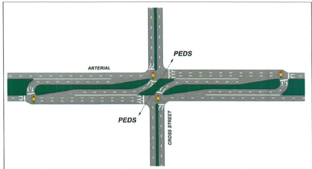
Figure 2. Superstreet Concept
