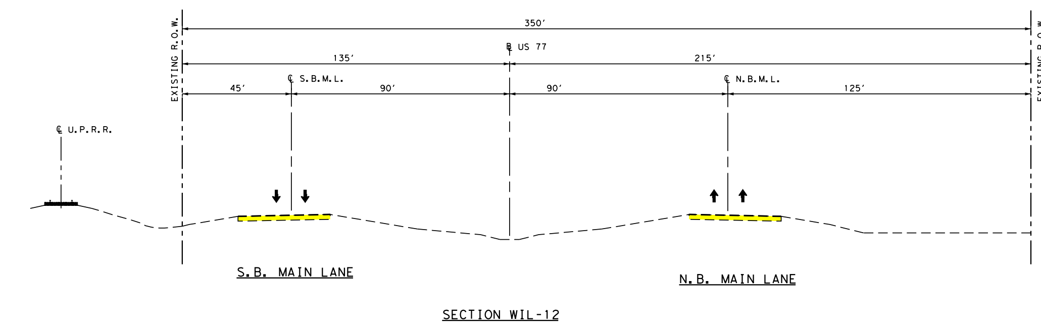
SECTION WIL-12
