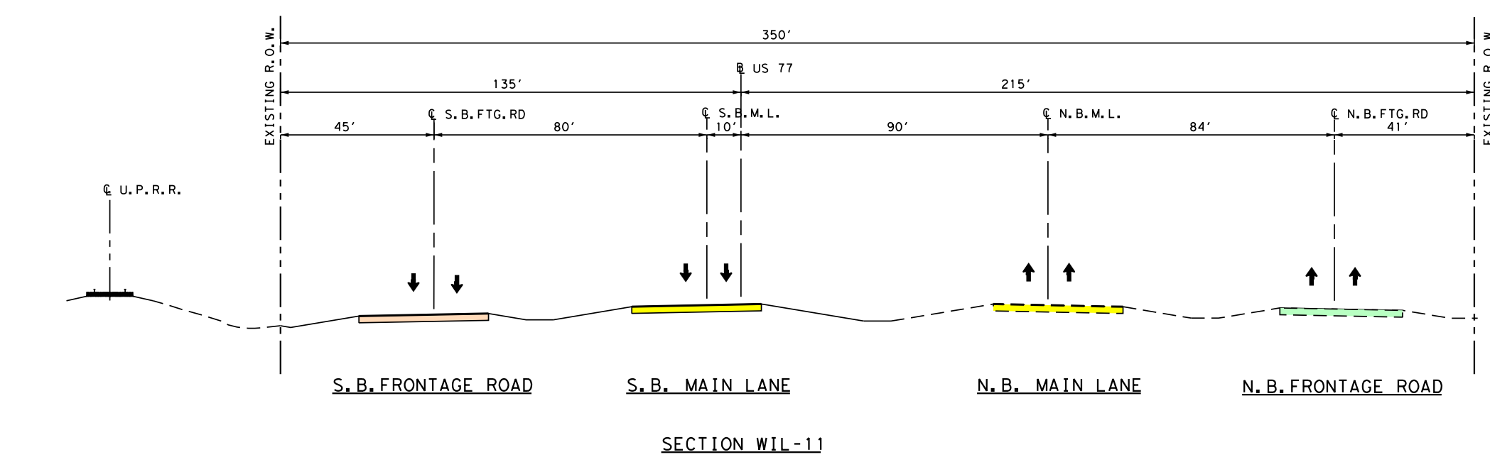
SECTION WIL-11
