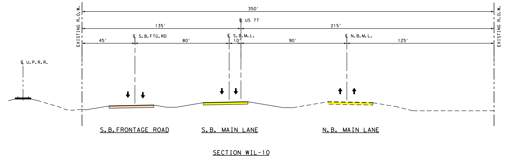
SECTION WIL-10
