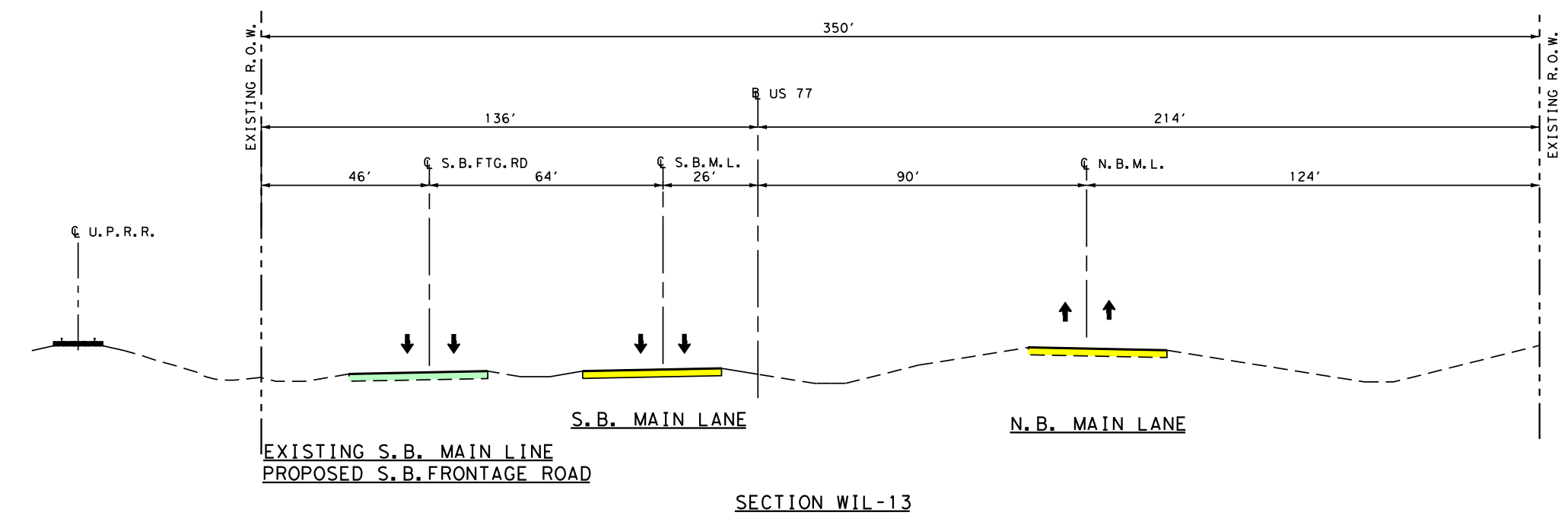
SECTION WIL-13
