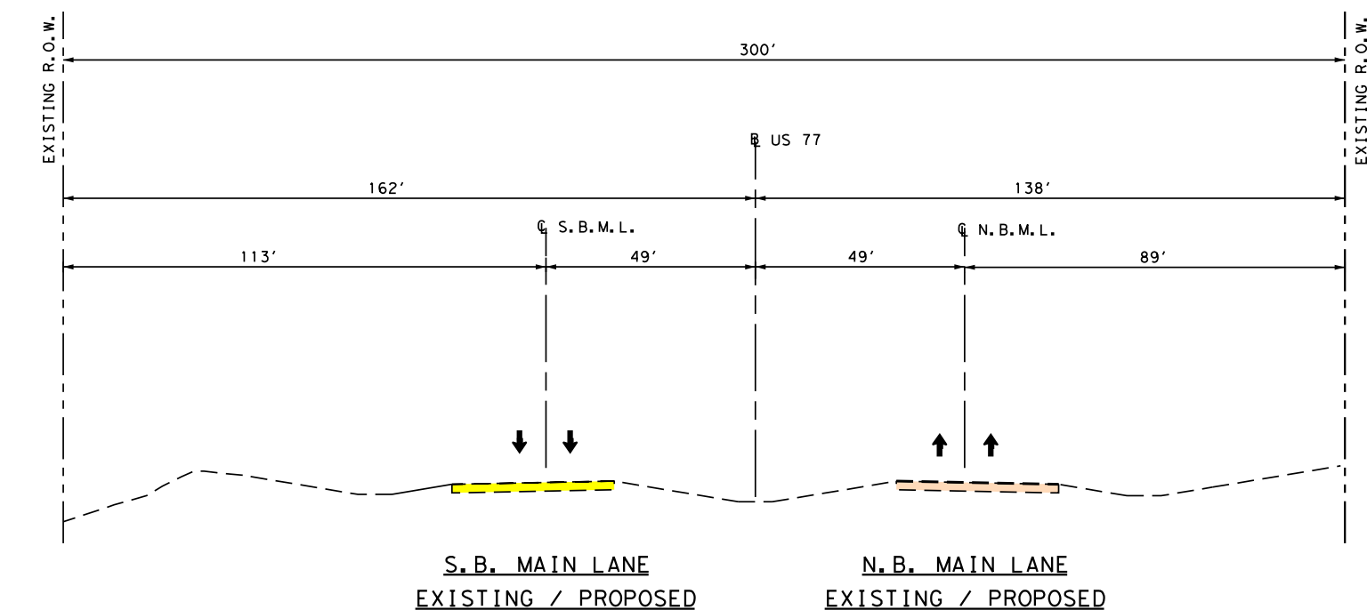
SECTION KLE-15
