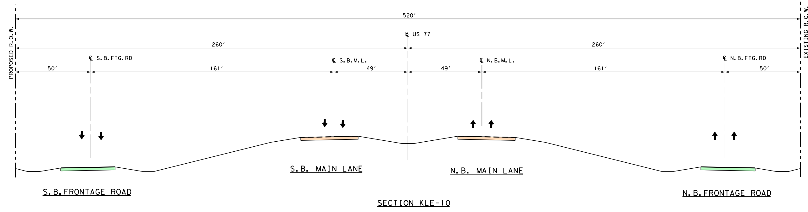
SECTION KLE-10
