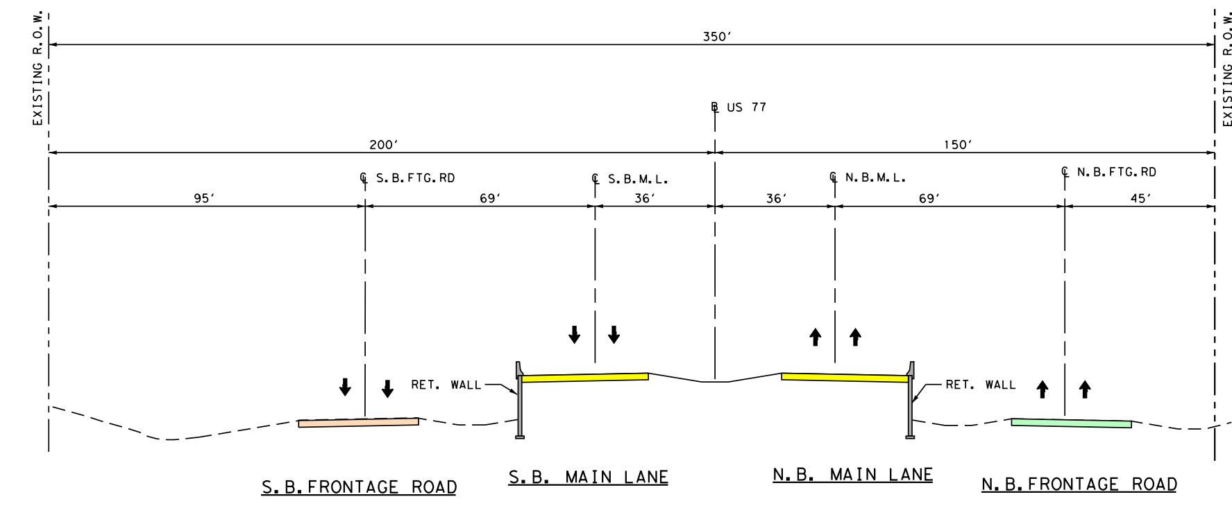
SECTION KLE-14
