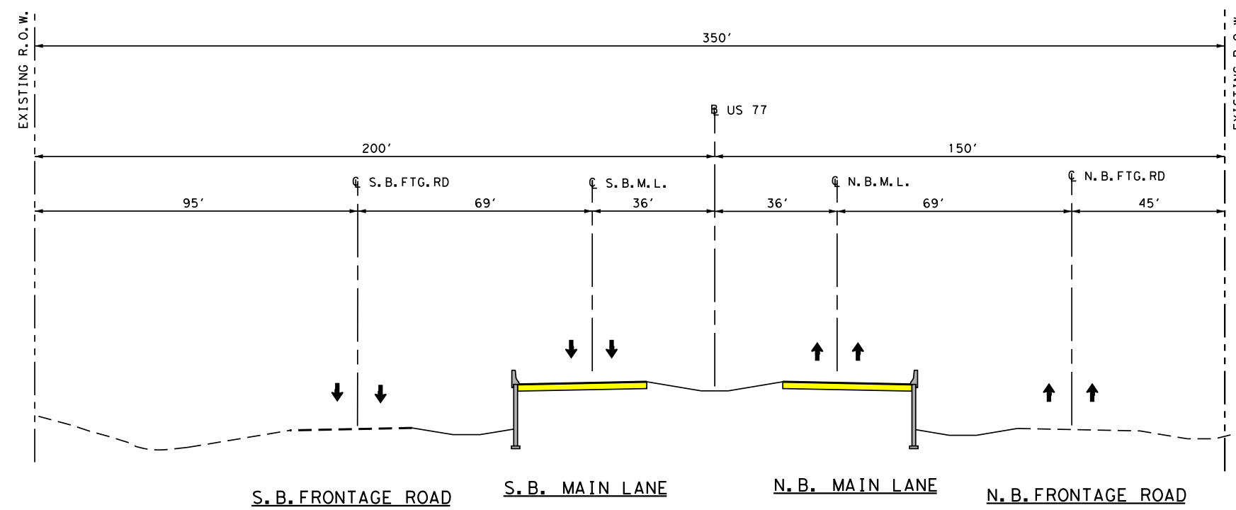
SECTION KLE-12
