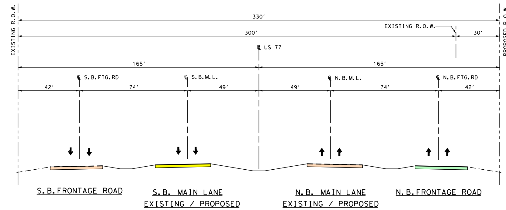
SECTION KLE-11
