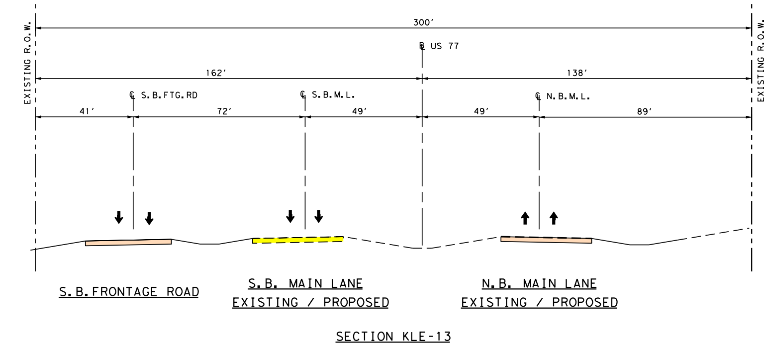
SECTION KLE-13
